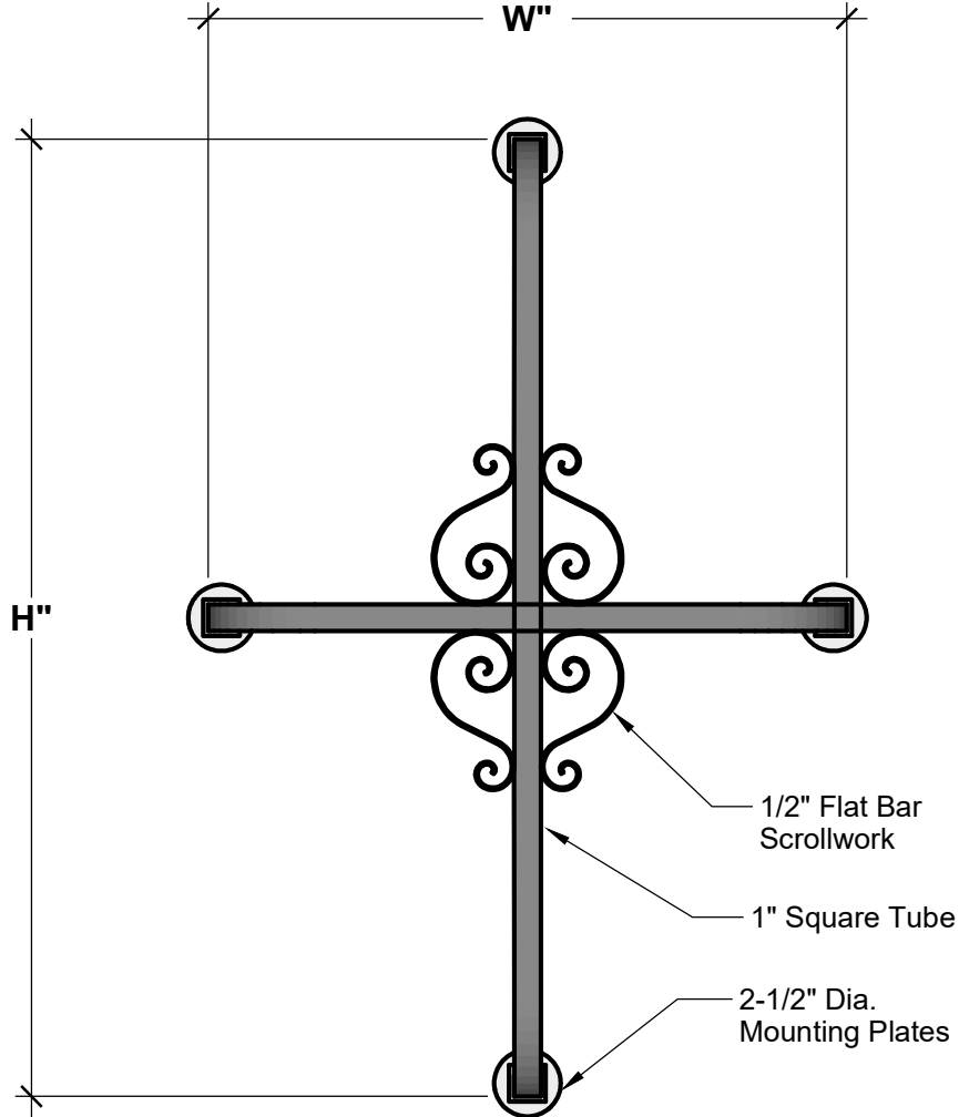
TOP VIEW
