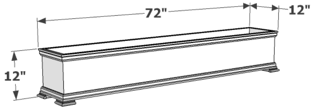
FRONT PERSPECTIVE
