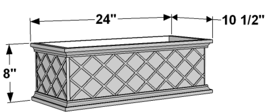
PERSPECTIVE VIEW
