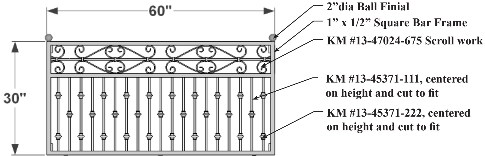
ELEVATION VIEW
