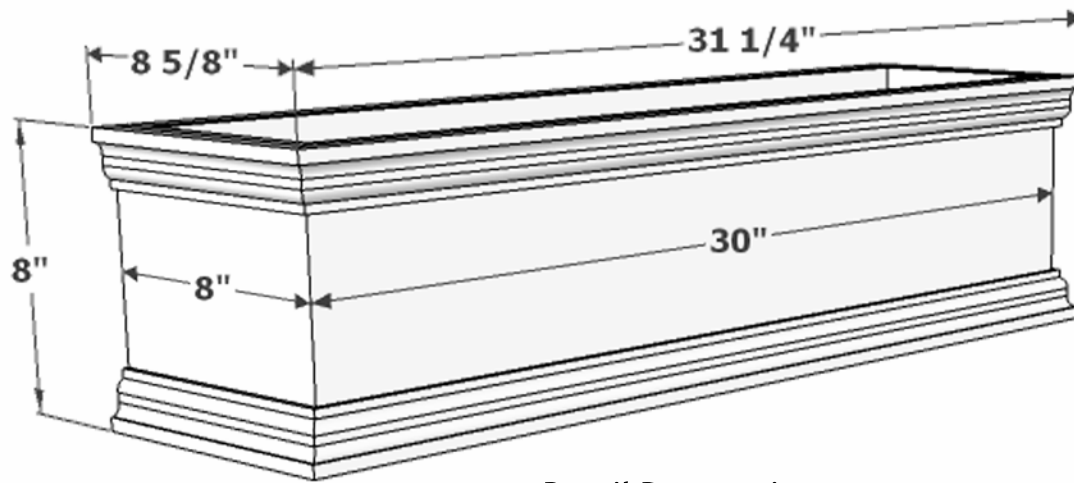
Detail Perspective
