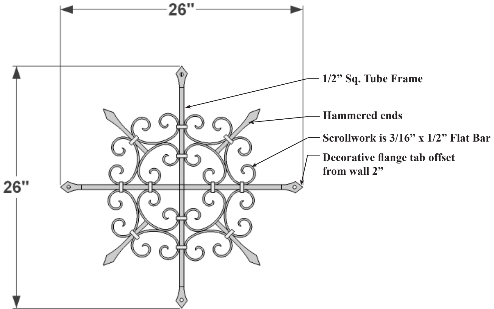
FRONT ELEVATION
