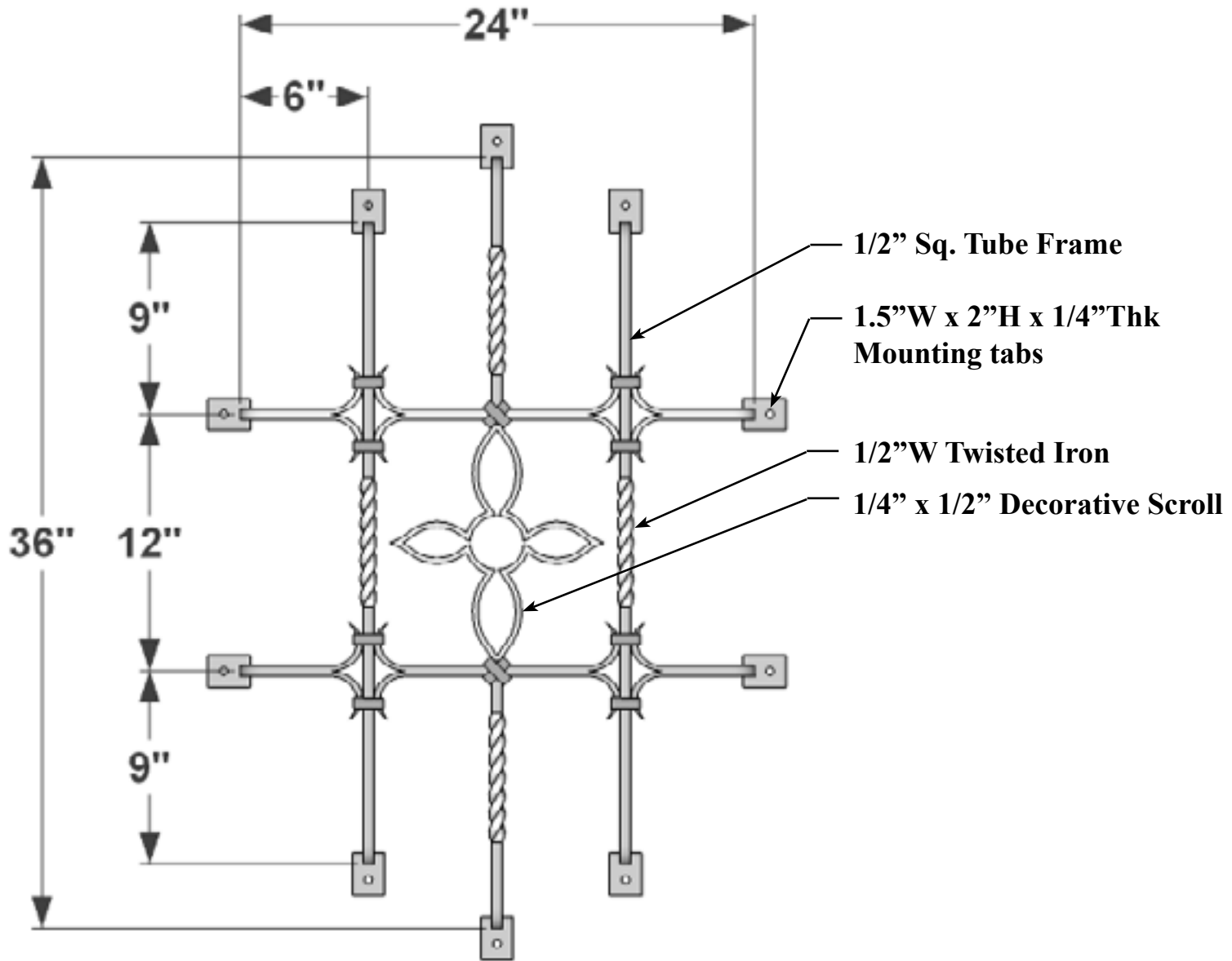
FRONT ELEVATION
