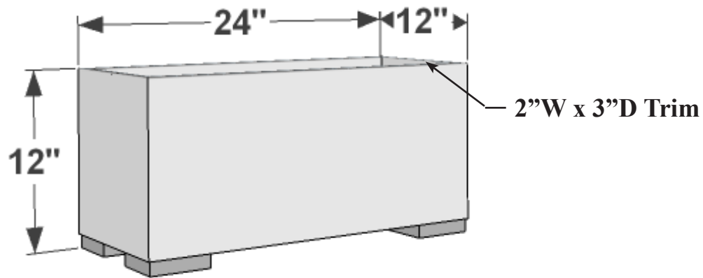
PERSPECTIVE VIEW
