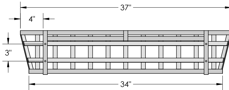
BACK VIEW
