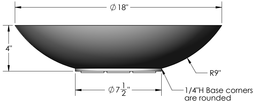
ELEVATION VIEW
